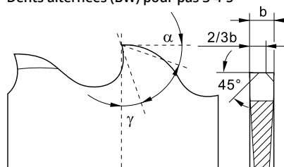
Denti sbazzatori finitori (C) 1 tooth for rough-hew / 1 tooth for finition 1 dents à degrossir / 1 dent a finition
